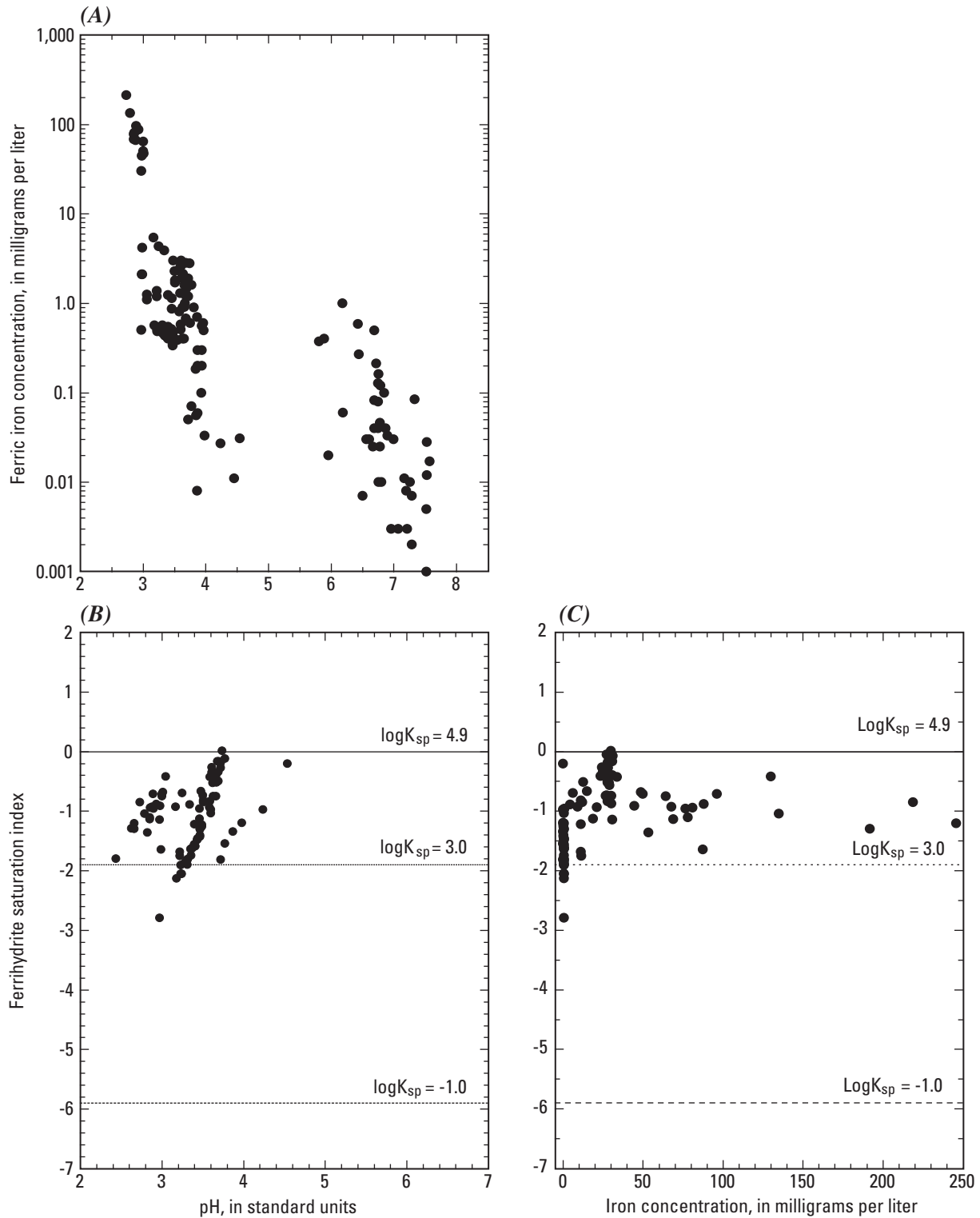
Figure 24. (A) Ferric iron concentrations plotted against pH for all ground waters and Straight Creek surface water. Ferrihydrite saturation index plotted against (B) pH and (C) iron for all ground waters and Straight Creek surface water fulfilling the Eh measurement requirements described in Naus and others (2005) and in Nordstrom and others (2005). The \log K_{sp} = 4.9 and 3.0 represent the upper and lower bounds, respectively, on the solubility of HFO (Nordstrom and others, 1990).
