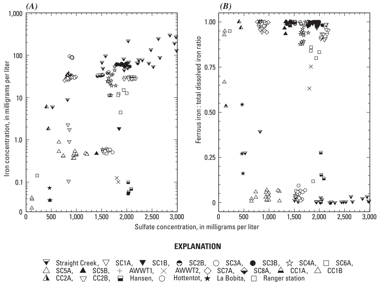
Figure 23. (A) Iron concentrations plotted against sulfate concentrations for all ground waters and Straight Creek surface water. (B) Ferrous iron:total dissolved iron molar ratio plotted against sulfate concentrations for all ground waters and Straight Creek surface water.
