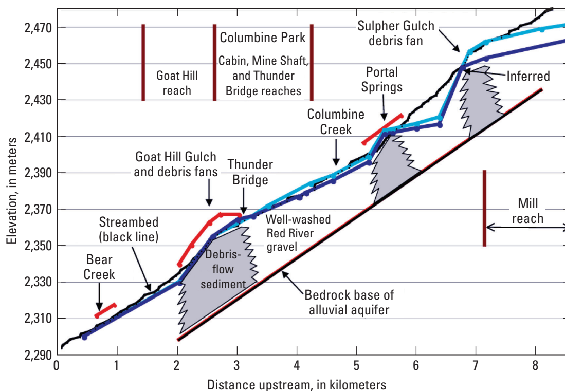
Figure 6. Longitudinal cross section of the Red River along the reach of the mine site projected onto a two-dimensional plane with bedrock surface, water tables (light blue for August 21, 2001, and dark blue for January–February 2002), projections of the debris-fan surface (red), and Red River streambed surface (from Vincent, in press).
