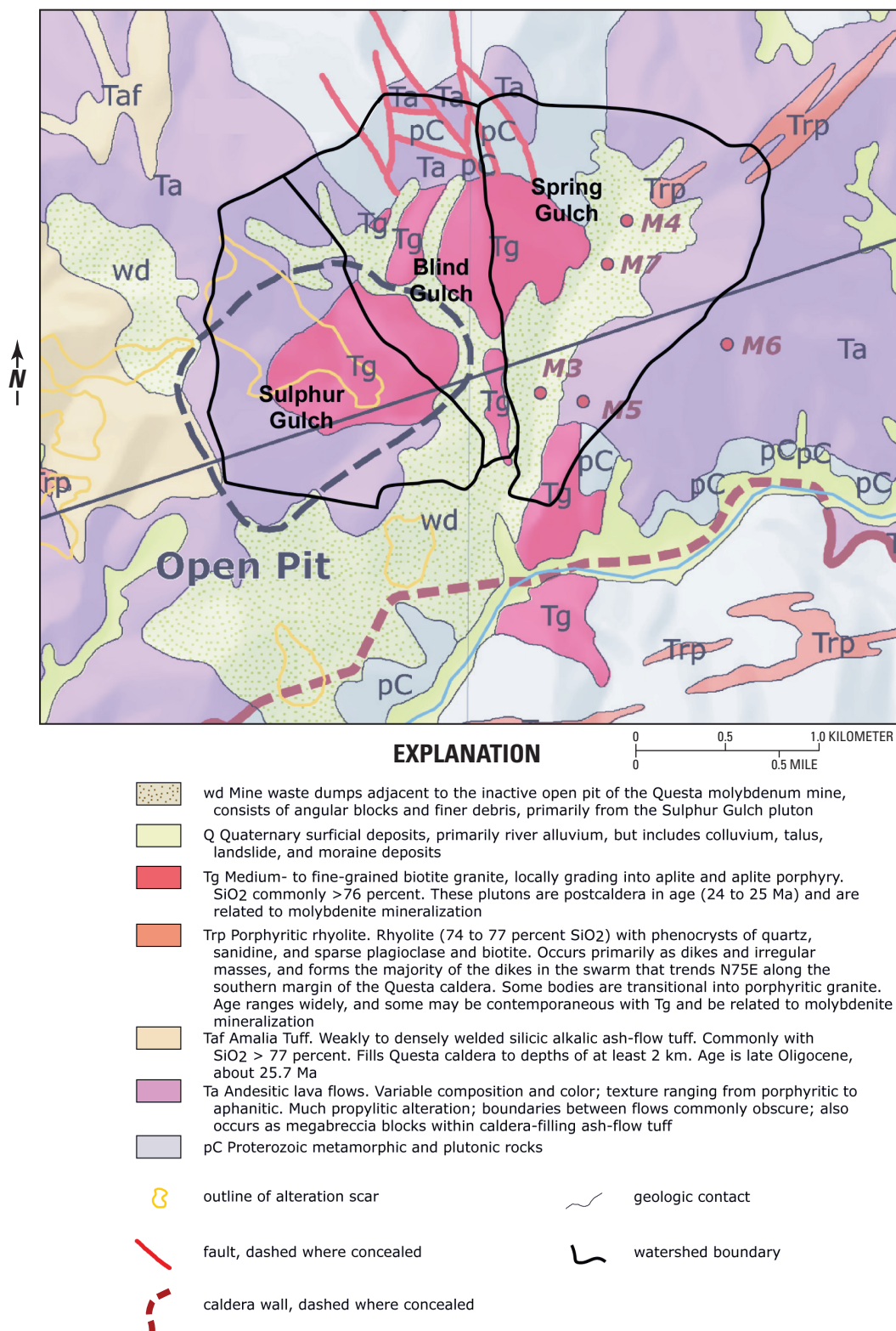
Figure 57. Geologic map of the three subcatchments that constitute Sulphur Gulch—upper Sulfur Gulch, Blind Gulch, and Spring Gulch.
