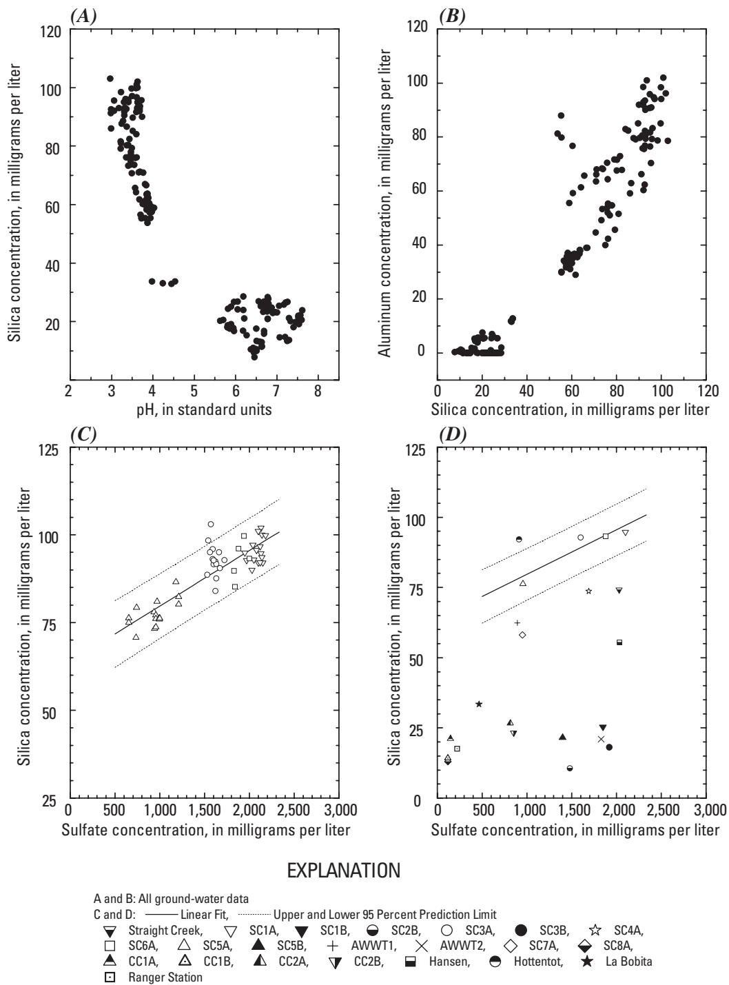
Figure 31. (A) Silica concentrations plotted against pH for all ground waters. (B) Silica concentrations plotted against aluminum concentrations for all ground waters. For samples having a pH value less than 4, silica concentrations plotted against sulfate concentrations for (C) Straight Creek alluvial ground water; and (D) median silica and sulfate concentrations for all ground waters and Straight Creek surface water. Linear fit and prediction limits at 95-percent probability for Straight Creek data only were used for both A and B (from Naus and others, 2005; Nordstrom and others, 2005).
