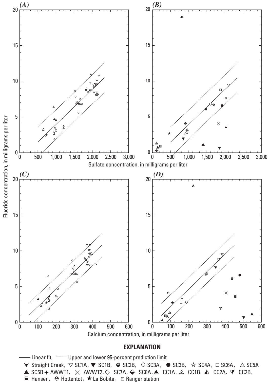
Figure 33. Fluoride concentrations plotted against sulfate concentrations for (A) Straight Creek alluvial ground waters and (B) median fluoride and sulfate concentrations for all ground waters and Straight Creek surface water. Fluoride concentrations plotted against calcium concentrations for (C) Straight Creek and alluvial ground water and (D) median concentrations for all ground waters and Straight Creek surface water. Linear fit and prediction limits at 95-percent probability for Straight Creek data only were used for all plots (from Naus and others, 2005; Nordstrom and others, 2005).
