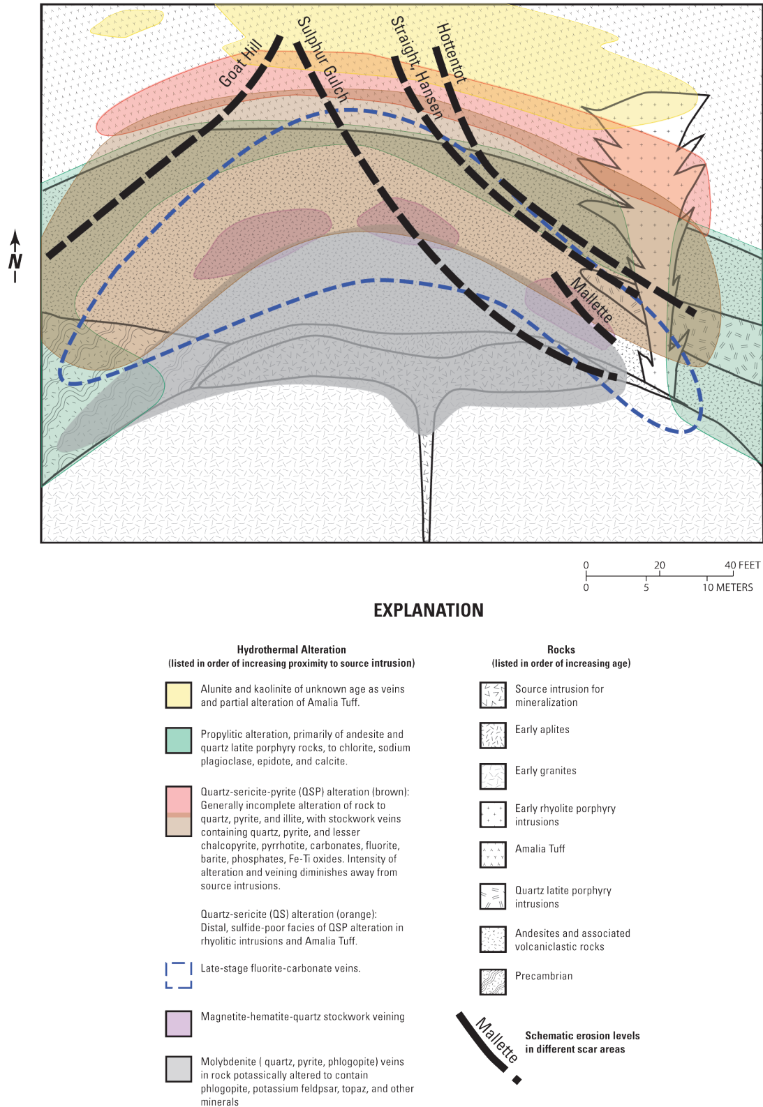
Figure 4. Schematic geologic cross section of alteration zones with overlying dashed lines depicting the relative position of the erosional surface for five catchments along the Red River (from Ludington and others, 2005).
