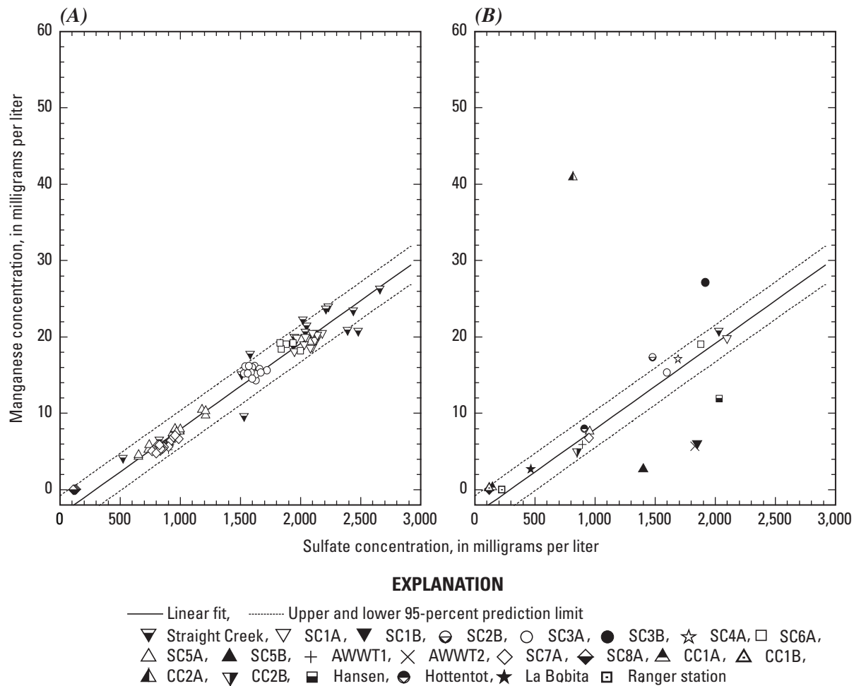
Figure 27. Manganese concentrations plotted against sulfate concentrations for (A) Straight Creek surface and alluvial ground waters and (B) median manganese and sulfate concentrations for all ground waters and Straight Creek surface water. Linear fit and prediction limits at 95-percent probability for Straight Creek data only were used for both A and B (from Naus and others, 2005; Nordstrom and others, 2005).
