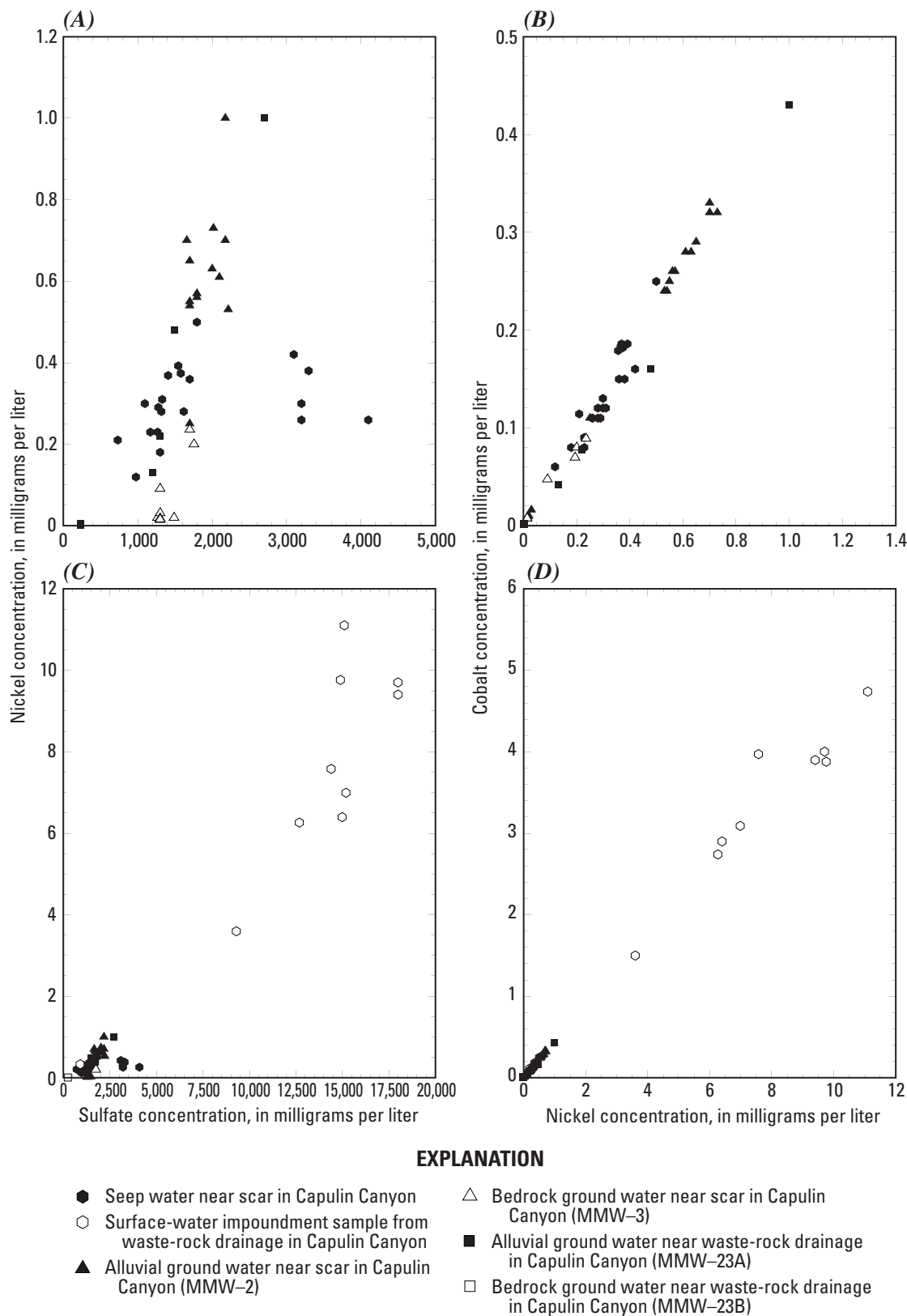
Figure 55. (A) Plot of nickel against sulfate concentrations (less than 5,000 milligrams per liter) for Capulin Canyon waters. (B) Plot of cobalt against nickel concentrations (less than 1.4 milligrams per liter) for Capulin Canyon waters. (C) Same plot as figure 55A but showing the entire range of concentrations. (D) Same plot as figure 55B but showing the entire range of concentrations.
