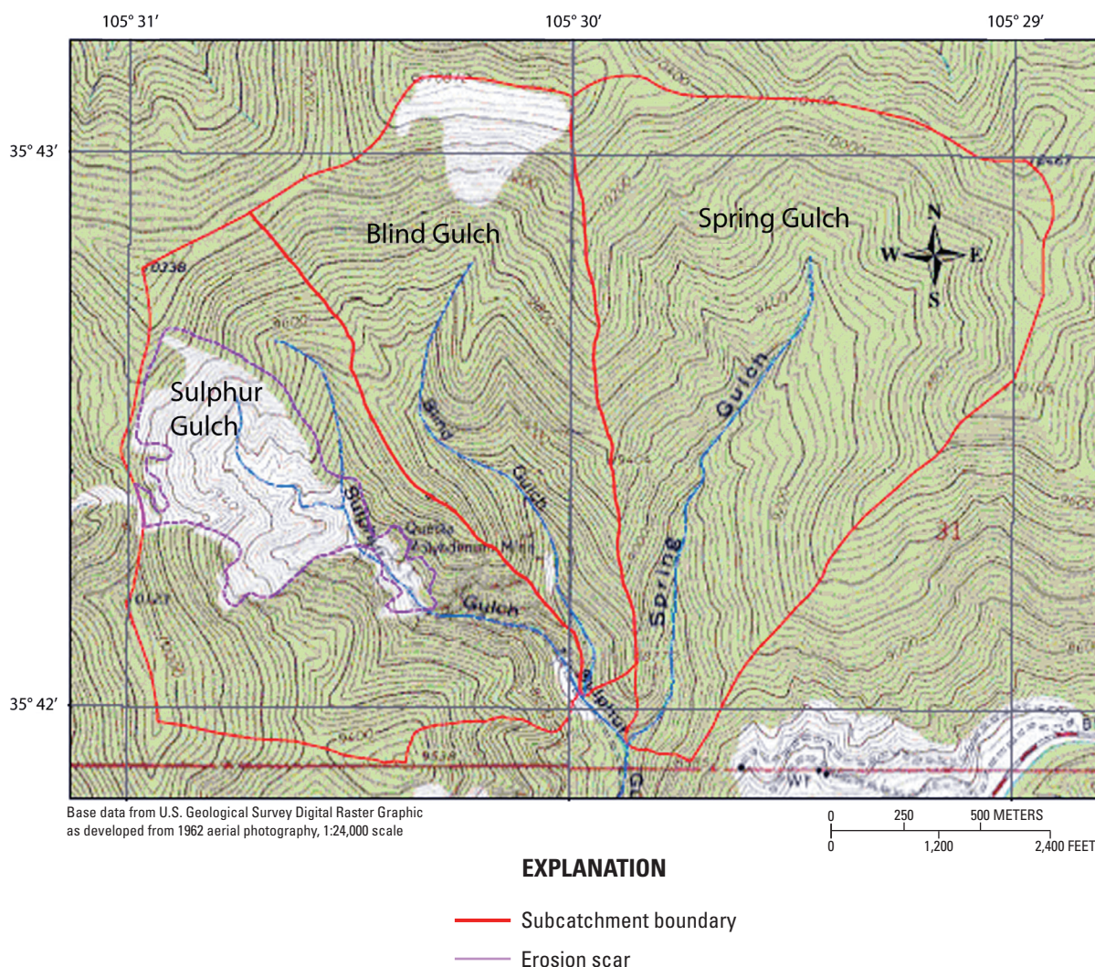
Figure 56. Topographic map of the three subcatchments that constitute Sulphur Gulch—upper Sulfur Gulch, Blind Gulch, and Spring Gulch.
