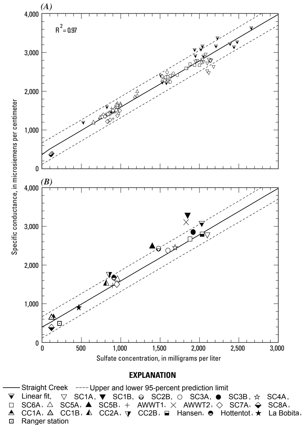
Figure 20. Plot of specific conductance against sulfate concentrations for (A) Straight Creek surface and alluvial ground waters and (B) median values for ground waters and Straight Creek surface water.
