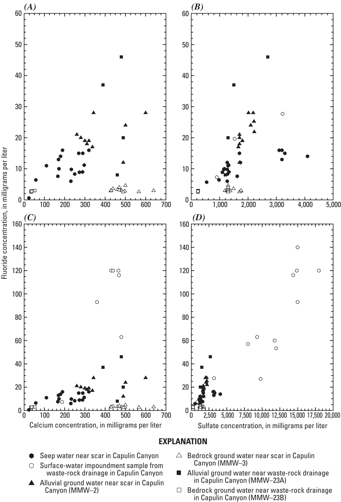
Figure 53. (A) Plot of fluoride concentrations (less than 60 milligrams per liter) against calcium concentrations for Capulin Canyon waters. (B) Plot of fluoride concentrations (less than 60 milligrams per liter) against sulfate concentrations (less than 5,000 milligrams per liter). (C) Same plot as figure 53A but showing the entire range of concentrations. (D) Same plot as figure 53B but showing the entire range of concentrations.
