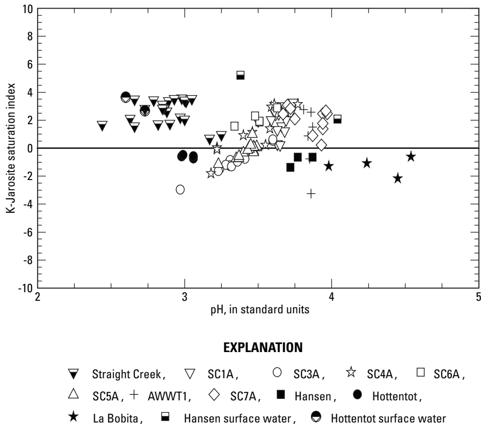
Figure 25. Saturation indices for potassium jarosite plotted relative to pH.
